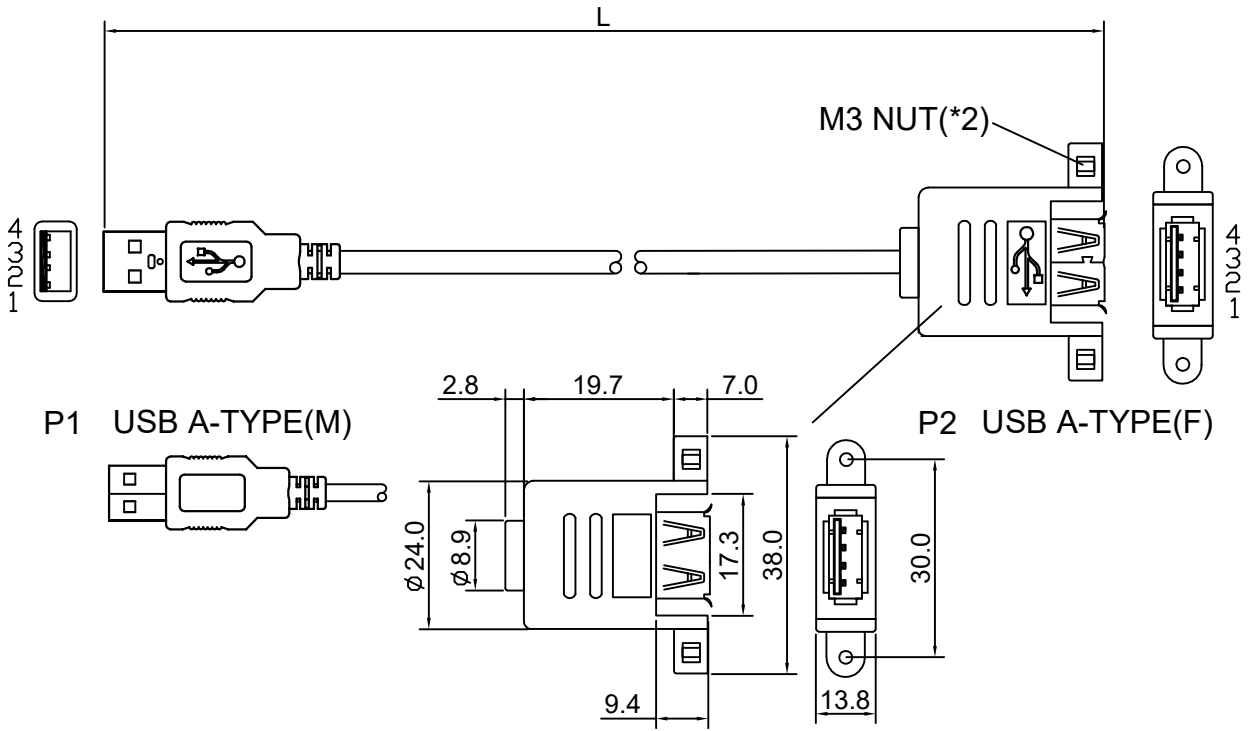
Wiring Diagram: Twisted
